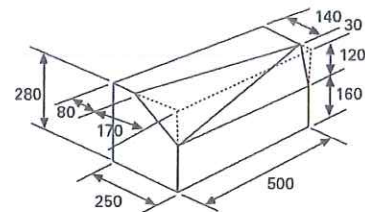
C BORDILLO REMONTABLE C-10 (CENTRAL)
